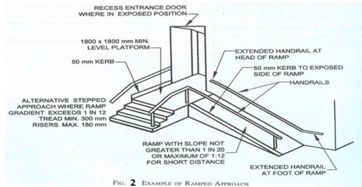
FIG. 2 EXAMPLE OF RAMPED APPROACH
